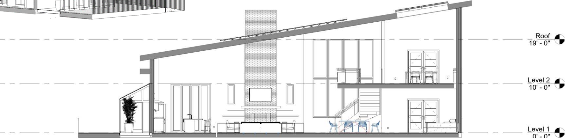
East/West Section
